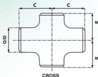
B16.9
