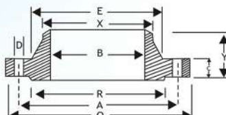
WELDING NECK FLANGE
