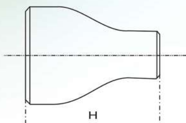
CONCENTRIC REDUCER
