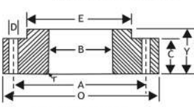
LAP JOINT FLANGE
