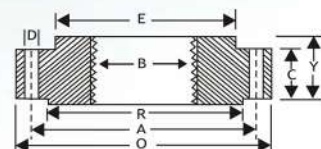
THREADED FLANGE
