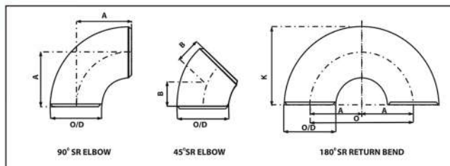
B16.9 / B16.28
