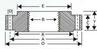
THREADED FLANGE
