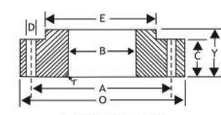
LAP JOINT FLANGE
