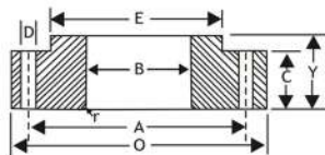
LAP JOINT FLANGE
