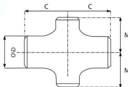
CROSS UNEQUAL
