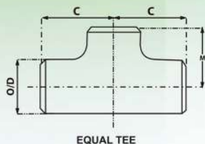
EQUAL TEE
