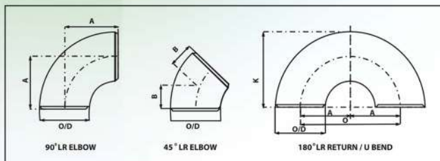
B16.9
