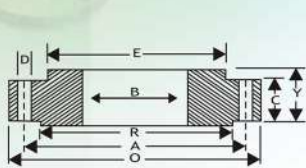
SLIP-ON FLANGE
