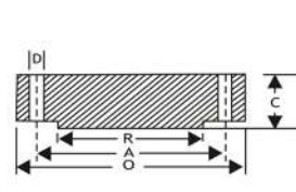
BLIND FLANGE
