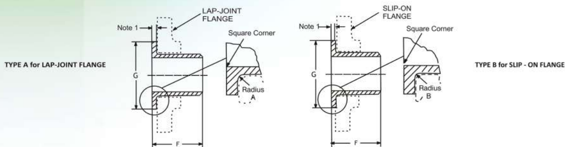
MSS SP 43
